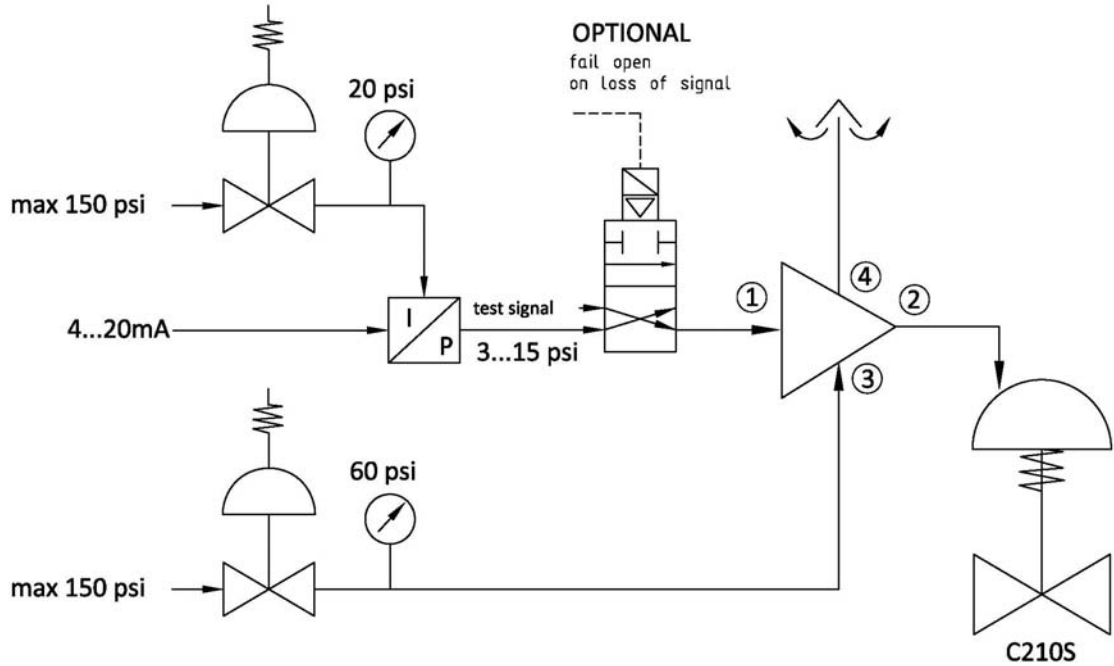
Fig. 8 Instrumentation schematic
