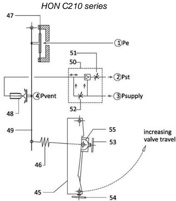
Fig. 6 Schematic diagram of the valve position
