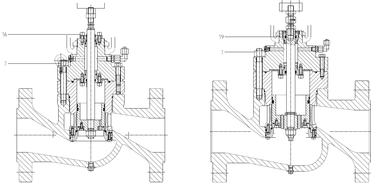
C210S 6"-12" CL150/600
